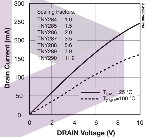
Figure 26. Output Characteristic.
